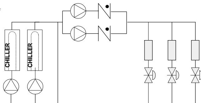
Fig. 1 Traditional primary/secondary system
