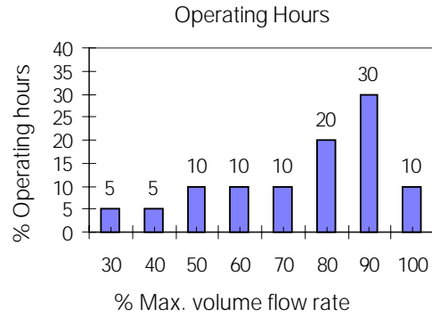
Fig. 5 Load Profile
