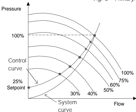
Figure 4: Variable Speed Pump Curves
