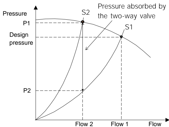
Fig. 2 Pressure absorbed by the two way valves
