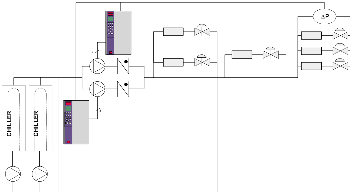
Fig. 3 - Primary/Secondary system with VLT frequency converters
