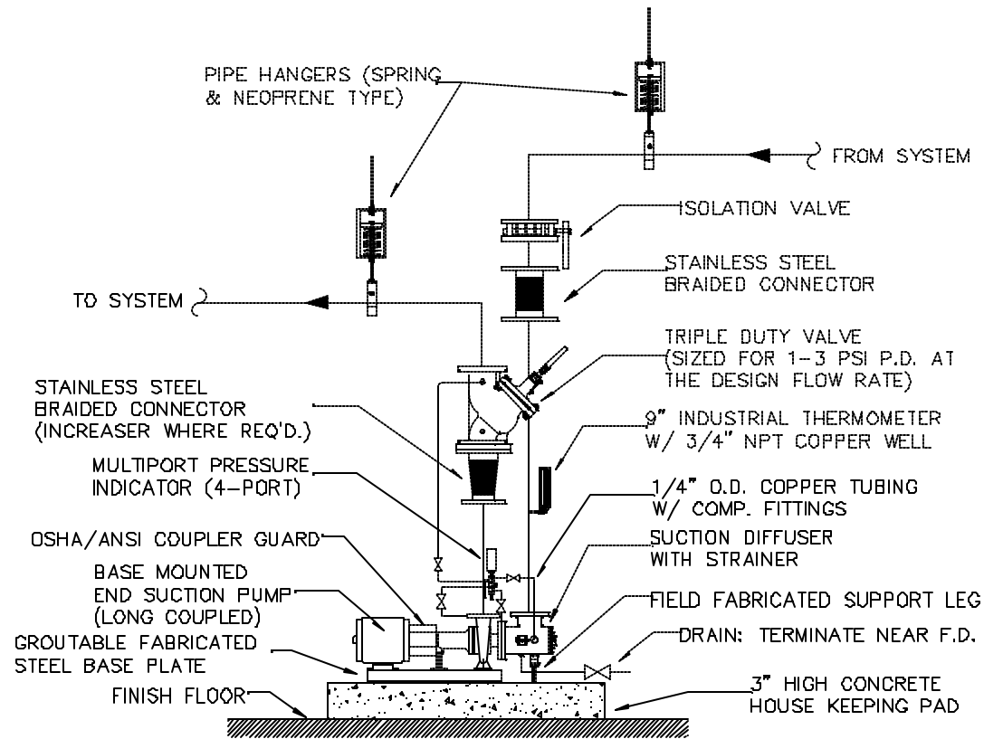
4 END SUCTION PUMP DETAIL - (BASE MOUNTED ON A HOUSEKEEPING PAD) NOT TO SCALE
