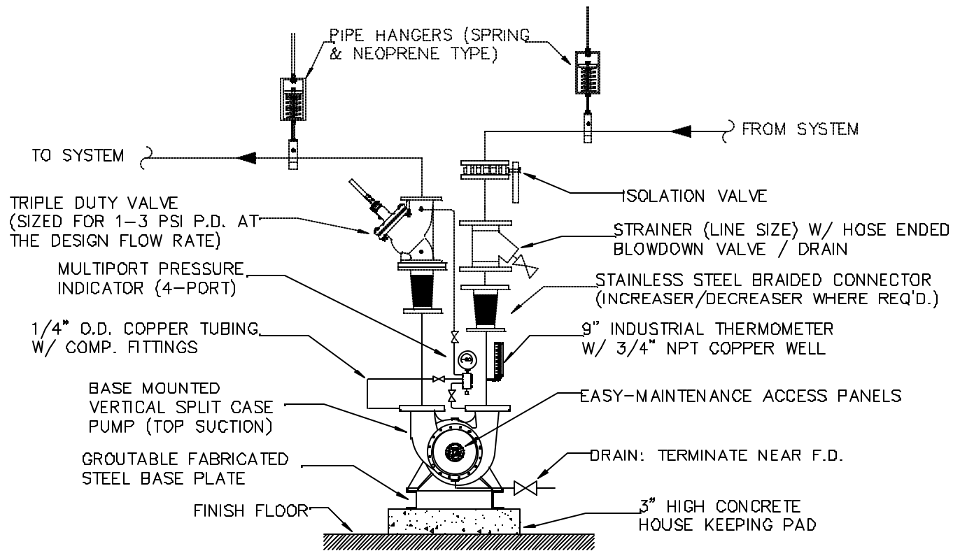
4 VERTICAL SPLIT CASE (TOP SUCTION) PUMP DETAIL — (BASE MOUNTED ON A HOUSEKEEPING PAD) NOT TO SCALE
