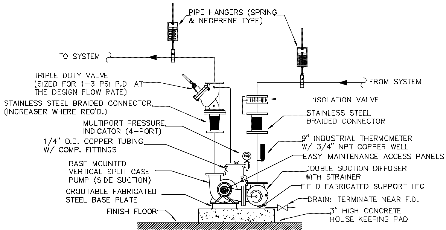
4 VERTICAL SPLIT CASE (SIDE SUCTION) PUMP DETAIL - (BASE MOUNTED ON A HOUSEKEEPING PAD) NOT TO SCALE
